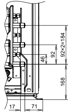
Side view (Valve part)
