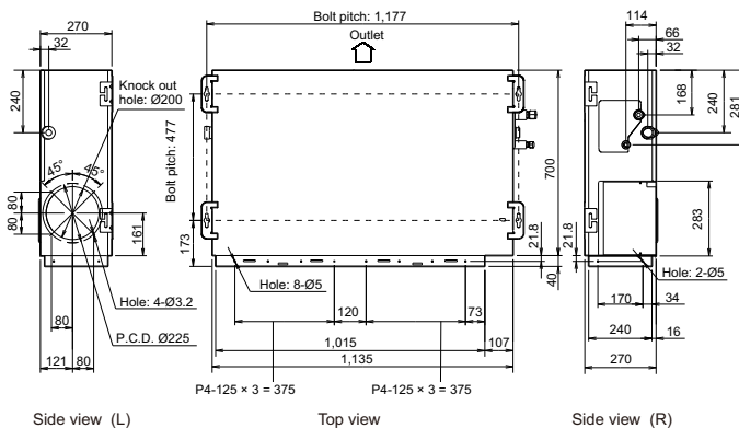
Side view (L)
