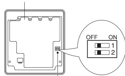
DIP Switch
